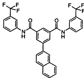
Compound # 18
